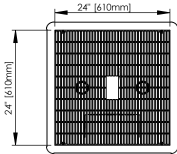
GRATE DETAIL
